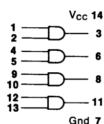
54/7408 Quad 2-input AND Gate
