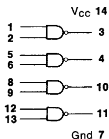
957 Quad 2-input Buffer
