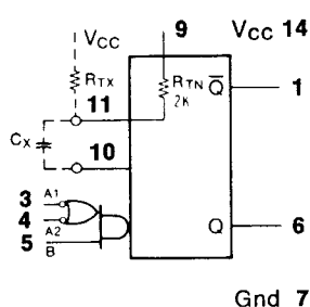
54/74121 Monostable Multivibrator
