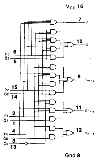
54/74182 Look-Ahead Carry Generator
