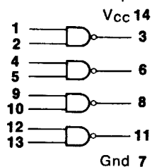
54/7403 Quad 2-input NAND Gate
