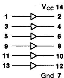
54/7407 Hex Buffer
