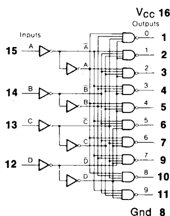
54/7443 EXCESS-3-to-Decimal Decoder
