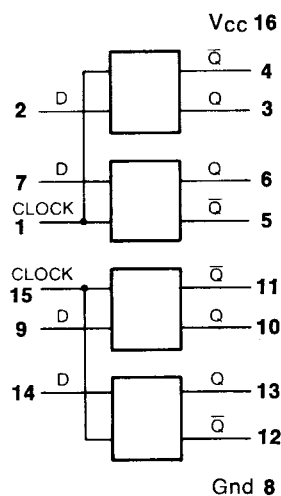
1813/1913 Quad Latch
