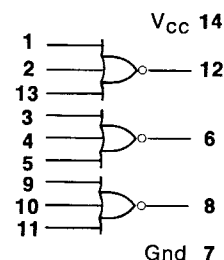
54/7427 Triple 3-input NOR Gate
