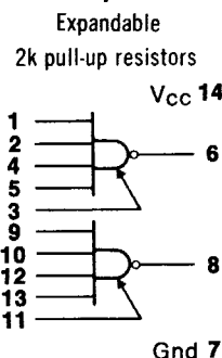
961 Dual 4-input NAND Gate
