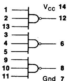
54/7410 Triple 3-input NAND Gate
