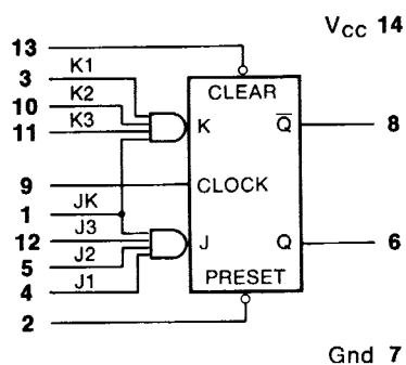
54/74104 Gated J-K Master-Slave Flip-Flop
