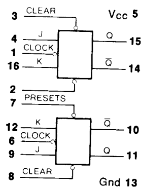
54/7476 Dual J-K Flip-Flop
