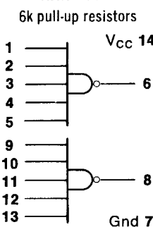
1800/1900 Dual 5-input NAND Gate
