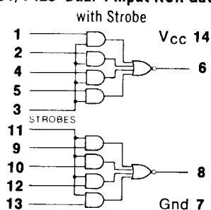
54/7425 Dual 4-input NOR Gate
