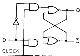
latch logic
