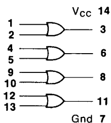
54/7432 Quad 2-input OR Gate
