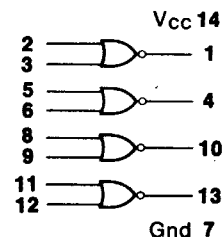
54/7402 Quad 2-input NOR Gate
