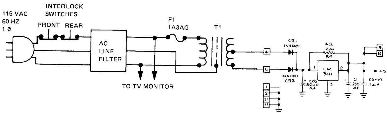
Figure 2-1. Power Supply
