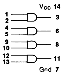
54/7409 Quad 2-input AND Gate
