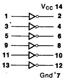
54/7404 Hex Inverter
