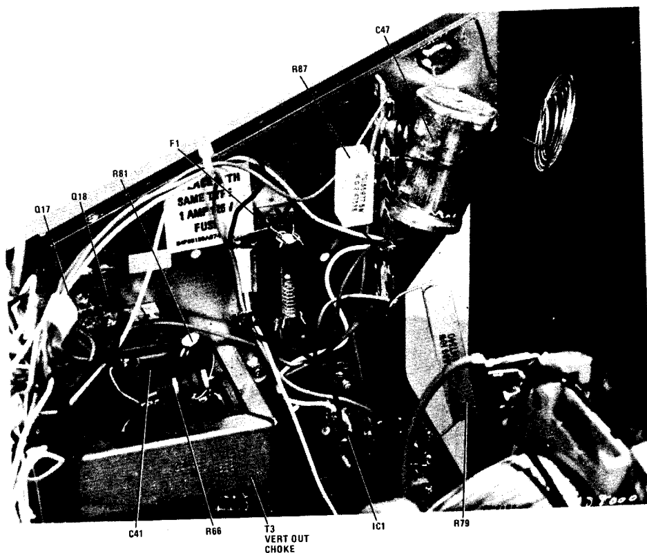
MODEL XM500-10 Right Side Panel – Component Location
