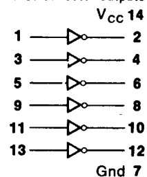
54/7405 Hex Inverter
