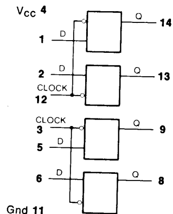
54/7477 Quad Latch *
