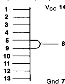
10-input NAND Gate 1804/1904 6k pull-up resistors 1805/1905 2k pull-up resistors
