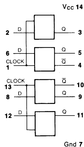
1814/1914 Quad Latch
