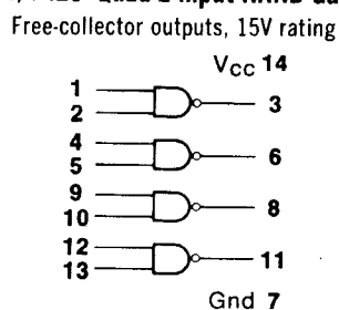
54/7426 Quad 2-input NAND Gate
