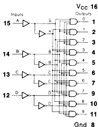
54/7442 BCD-to-Decimal Decoder
