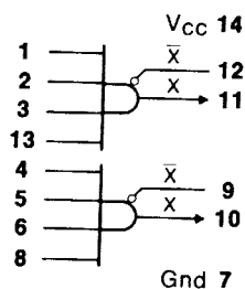
54/7460 Dual AND-OR Expander
