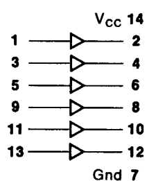
54/7417 Hex Buffer
