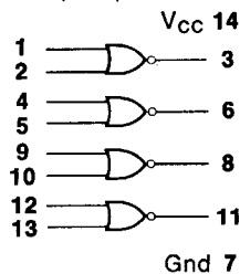
1810/1910 Quad 2-input NOR Gate 6k pull-up resistors
