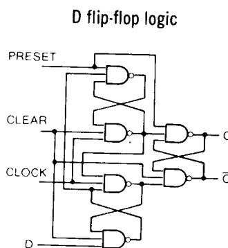
54/7474 Dual D Flip-Flop
