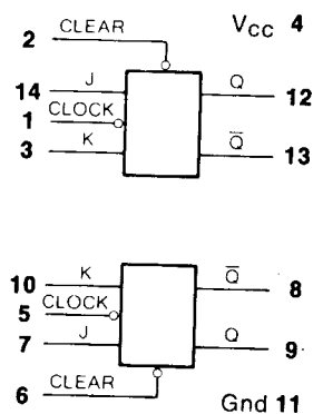
54/7473 Dual J-K Flip-Flop
