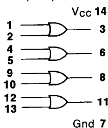
1808/1908 Quad 2-input OR Gate 6k pull-up resistors
