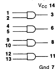
Quad 2-input AND Gate 1806/1906 6k pull-up resistors 1807/1907 2k pull-up resistors
