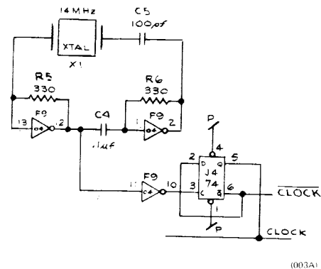
Figure 2-2. Computer Clock
