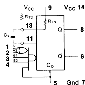
54/74122 Retriggerable Multivibrator
