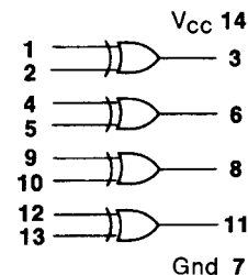
1812/1912 Quad Exclusive-OR Gate 6k pull-up resistors
