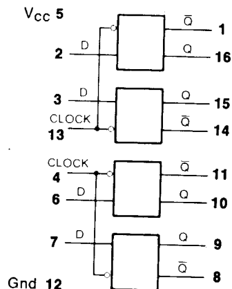
54/7475 Quad Latch
