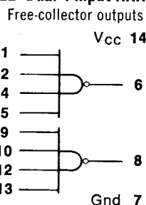
54/7422 Dual 4-input NAND Gate
